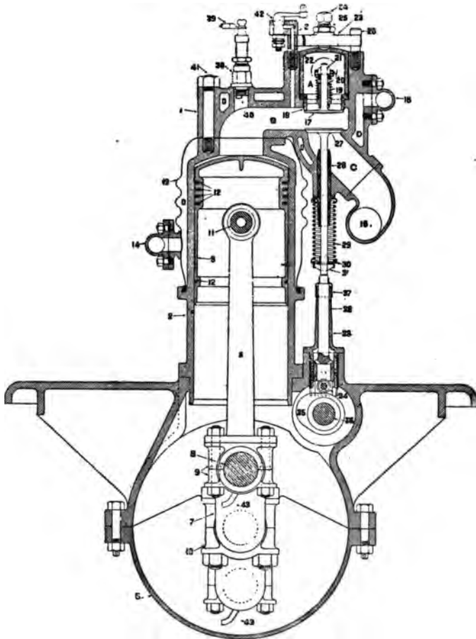
FIG. 24.—Section through One Cylinder of an Automobile Engine (Pope-Toledo), operated by automatic inlet. The parts are: 1, cylinder head; 2, cylinder; 3, piston; 4, crank case, upper half; 5, crank case, lower half; 6, connecting rod; 7, crank arm; 8, crank pin; 9, crank brasses; 10, crank shaft bearing; 11, piston pin; 12, piston rings; 13, water jacket casing; 14, water inlet pipe; 15, water outlet pipe; 16, exhaust pipe; 17, inlet valve; 18, inlet valve seating; 19, inlet valve spring; 20, inlet valve spring retainer; 21, inlet valve spring retainer key; 22, inlet valve cap; 23, inlet valve yoke; 24, inlet valve set screw; 25, inlet valve set screw lock nut; 26, inlet valve yoke stub; 27, exhaust valve; 28, exhaust valve stem bushing; 29, exhaust valve spring; 30, exhaust valve spring retainer; 31, exhaust valve spring retainer key; 32, exhaust valve push rod; 33, exhaust valve push rod guide; 34, exhaust cam roller; 35, exhaust cam; 36, exhaust cam shaft; 37, dust cap; 38, sparking plug; 39, sparking terminal; 40, spark points; 41, cylinder head studs; 42, relief cock; 43, oil scoop; A, inlet chamber; B, compression space; C, exhaust passage; D, water space.
